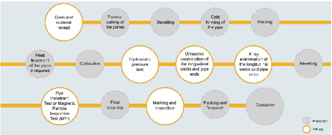
Manufacturing route of metallurgically clad pipes
